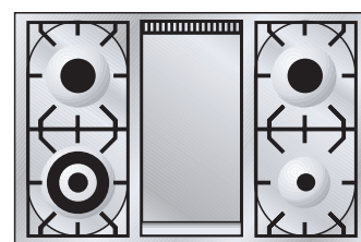
90cm Nostalgie 5 Burner Model PN90FVG Total Electrical Load (Kw) 2.45 Total Gas 'NG' Consumption (Mj/h) 70
