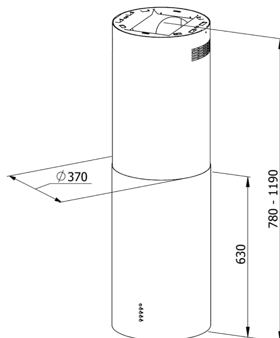
Model: X370 Island Hood Size: 37cm diameter Power standard: 10 Amp plug Ducting size: 150mm
